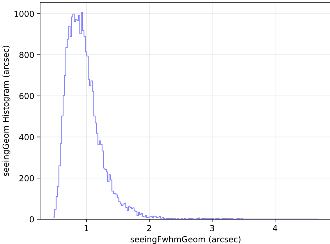
too_elab_r64_d3_ugrizy_v3.4_10yrs Yr 1 g band: seeingGeom Histogram
