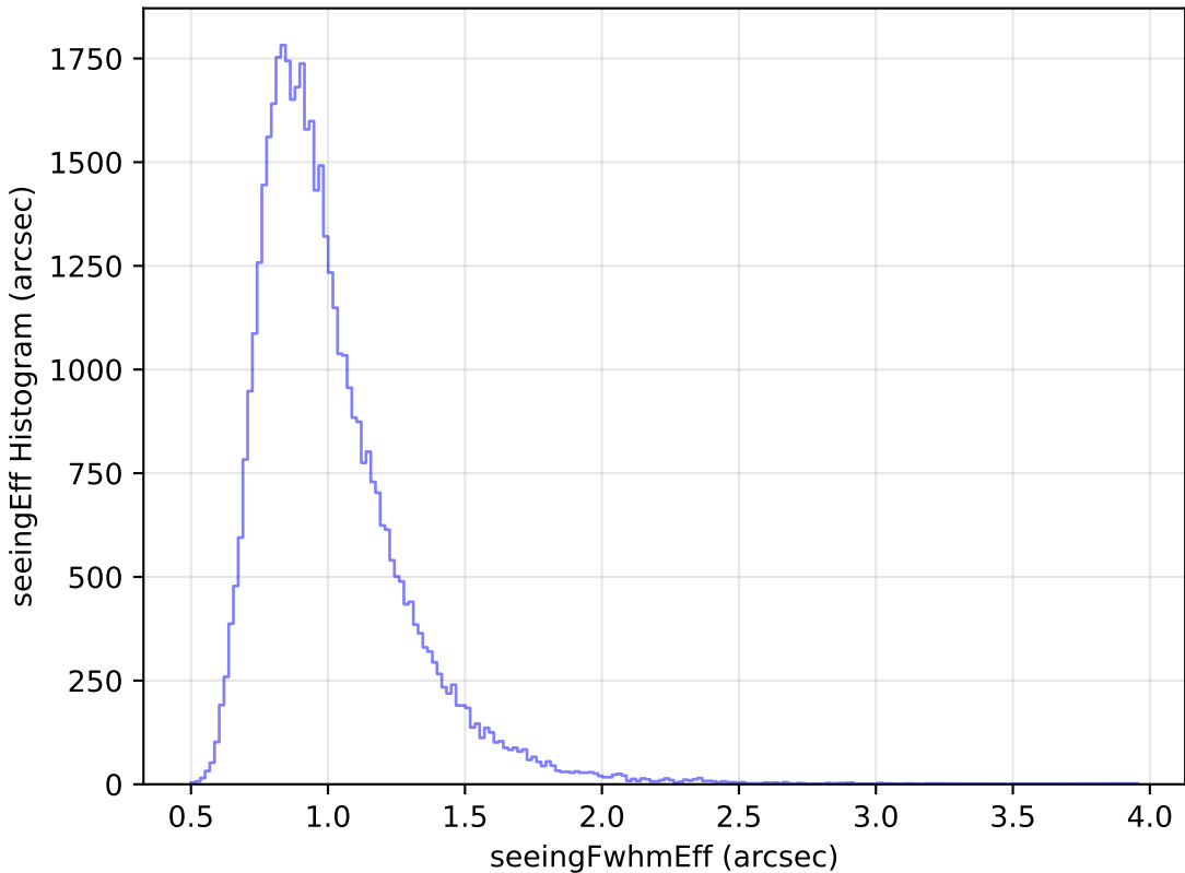
too_elab_r64_d3_ugrizy_v3.4_10yrs Yr 1 y band: seeingEff Histogram
