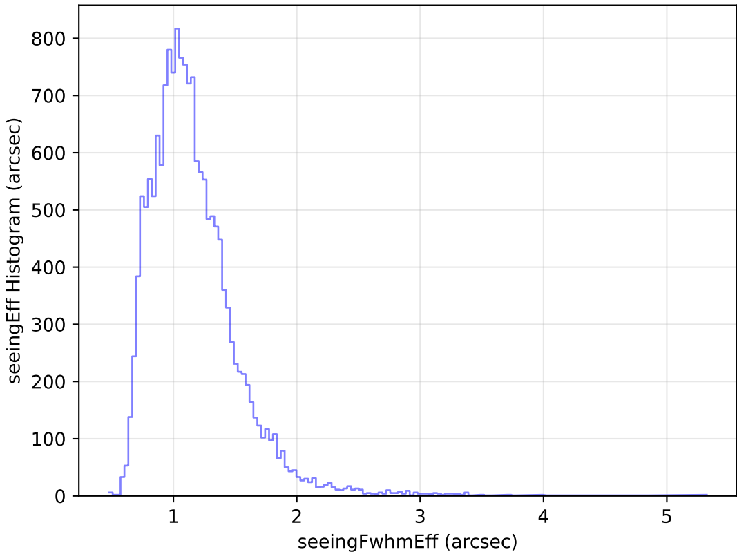
too_elab_r64_d3_ugrizy_v3.4_10yrs Yr 1 u band: seeingEff Histogram
