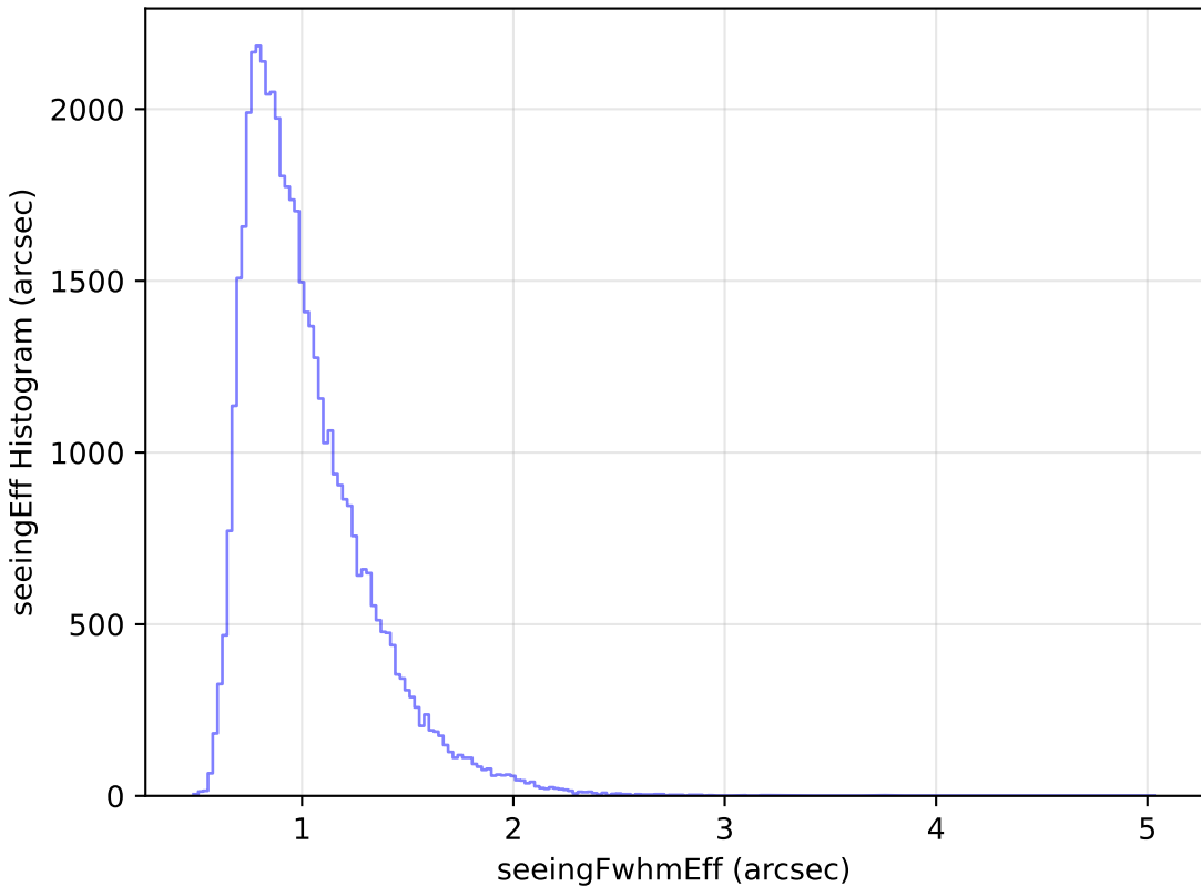
too_elab_r64_d3_ugrizy_v3.4_10yrs Yr 1 r band: seeingEff Histogram
