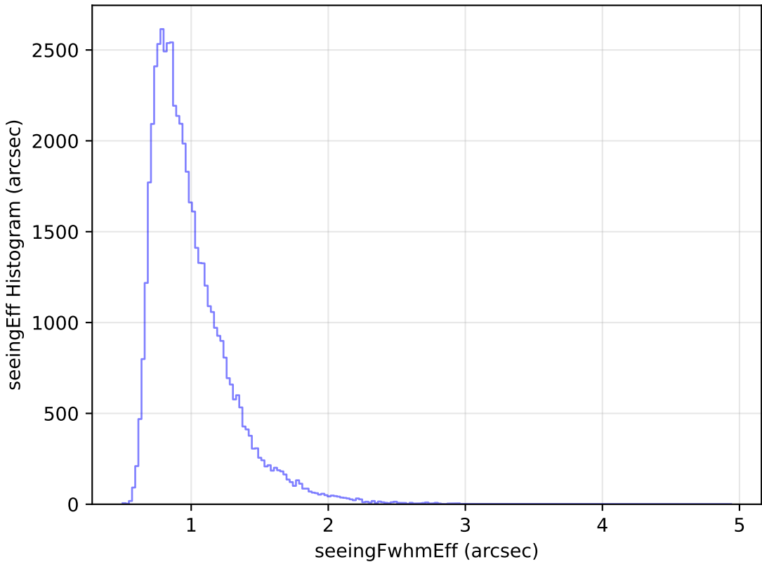
too_elab_r64_d3_ugrizy_v3.4_10yrs Yr 1 i band: seeingEff Histogram
