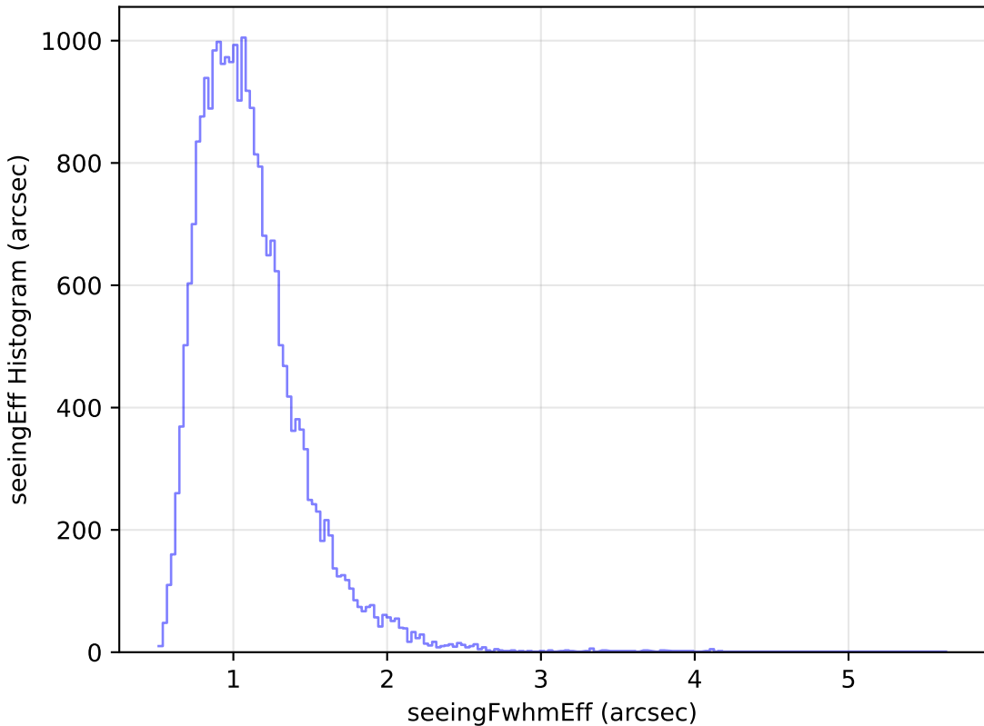
too_elab_r64_d3_ugrizy_v3.4_10yrs Yr 1 g band: seeingEff Histogram
