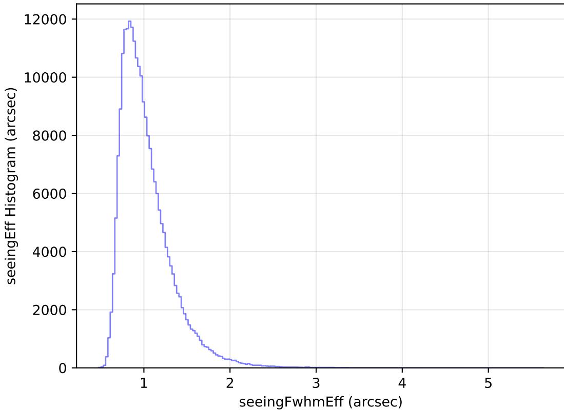
too_elab_r64_d3_ugrizy_v3.4_10yrs Yr 1 all bands: seeingEff Histogram
