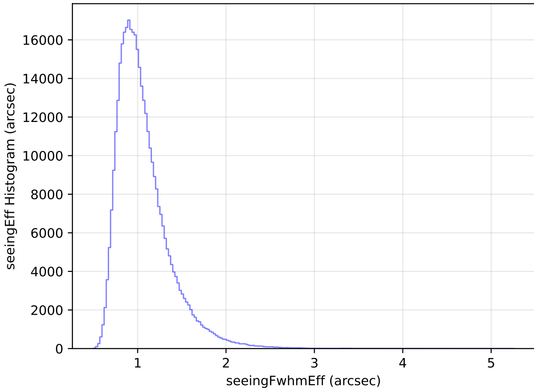
too_elab_r64_d3_ugrizy_v3.4_10yrs WFD y band: seeingEff Histogram
