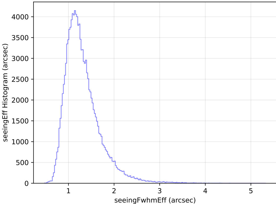
too_elab_r64_d3_ugrizy_v3.4_10yrs WFD u band: seeingEff Histogram
