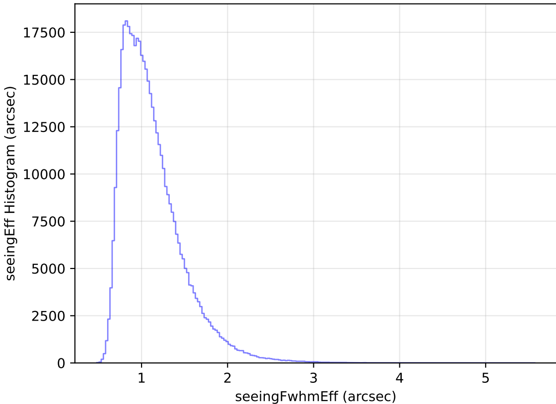
too_elab_r64_d3_ugrizy_v3.4_10yrs WFD r band: seeingEff Histogram
