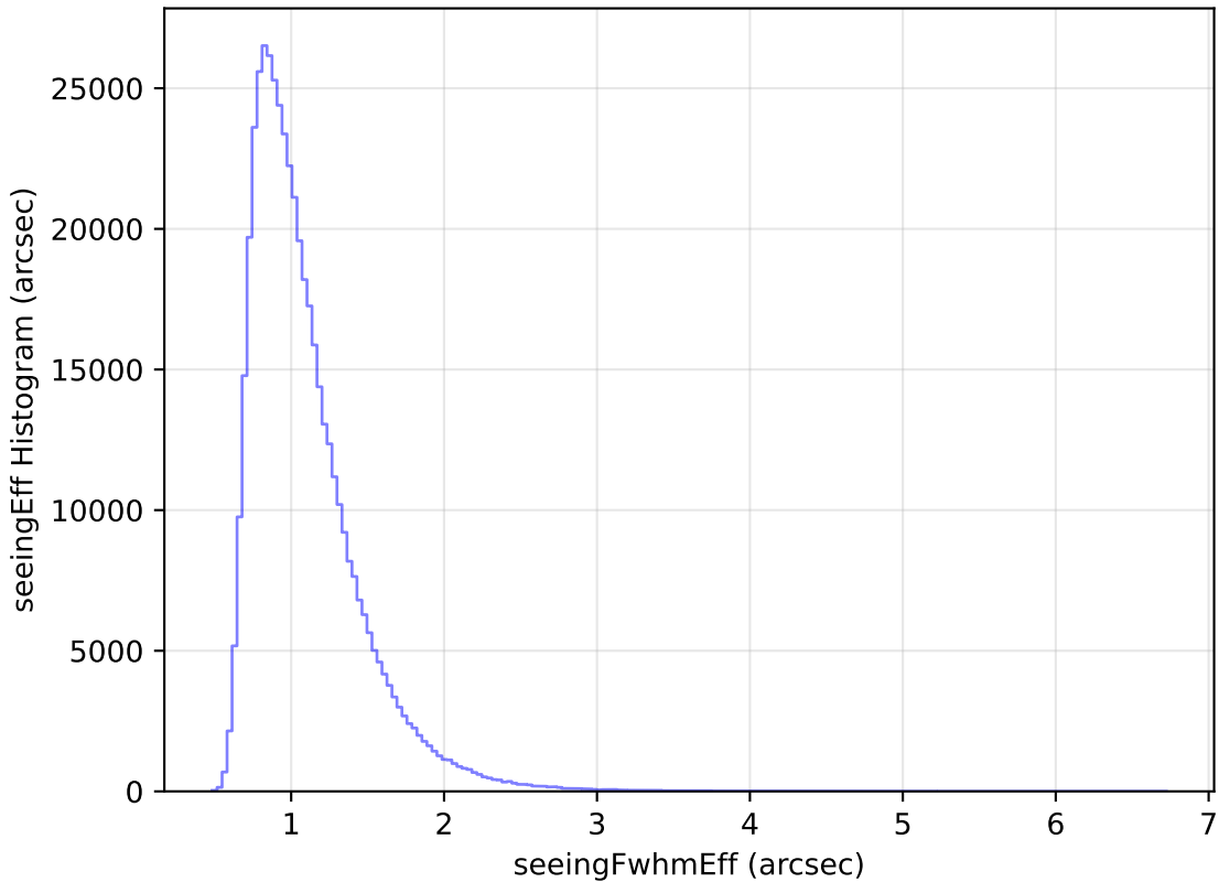
too_elab_r64_d3_ugrizy_v3.4_10yrs WFD i band: seeingEff Histogram
