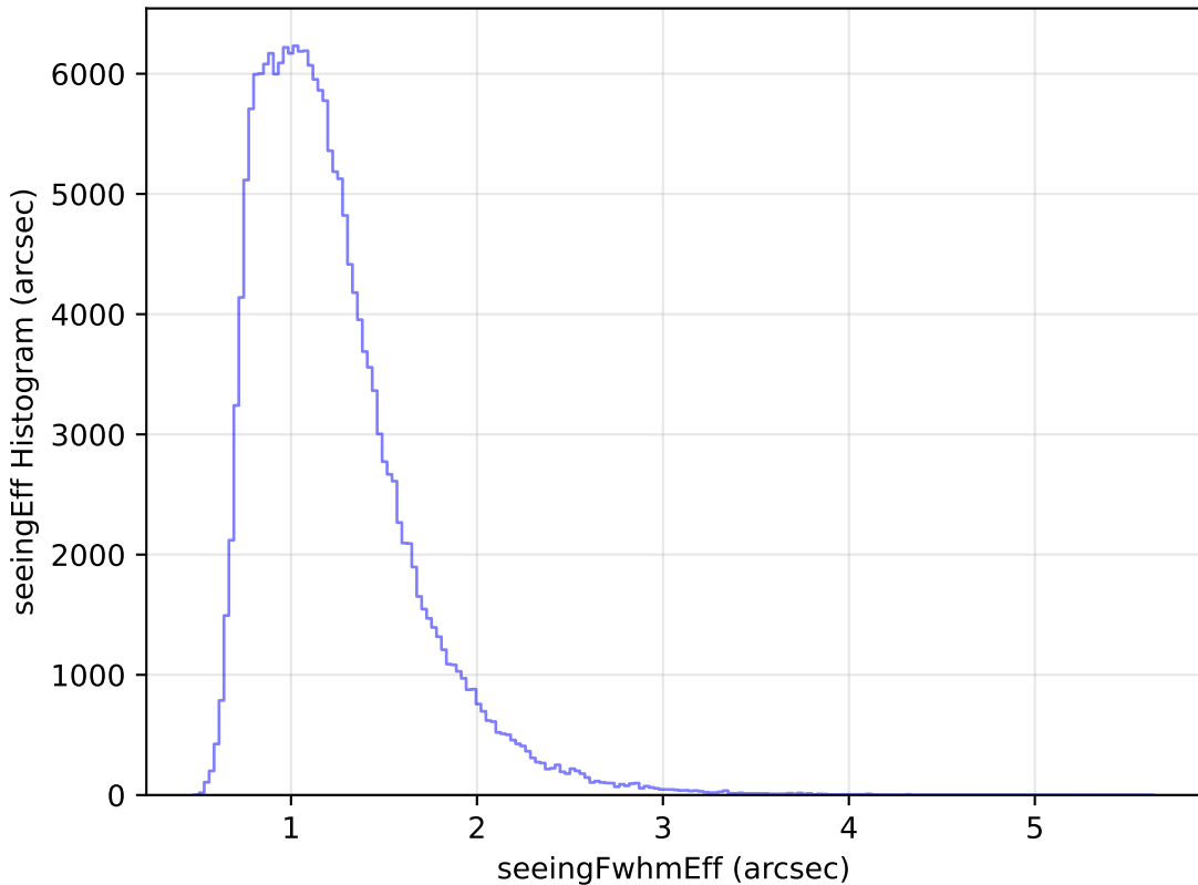
too_elab_r64_d3_ugrizy_v3.4_10yrs WFD g band: seeingEff Histogram
