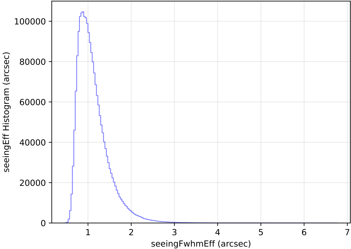
too_elab_r64_d3_ugrizy_v3.4_10yrs WFD all bands: seeingEff Histogram
