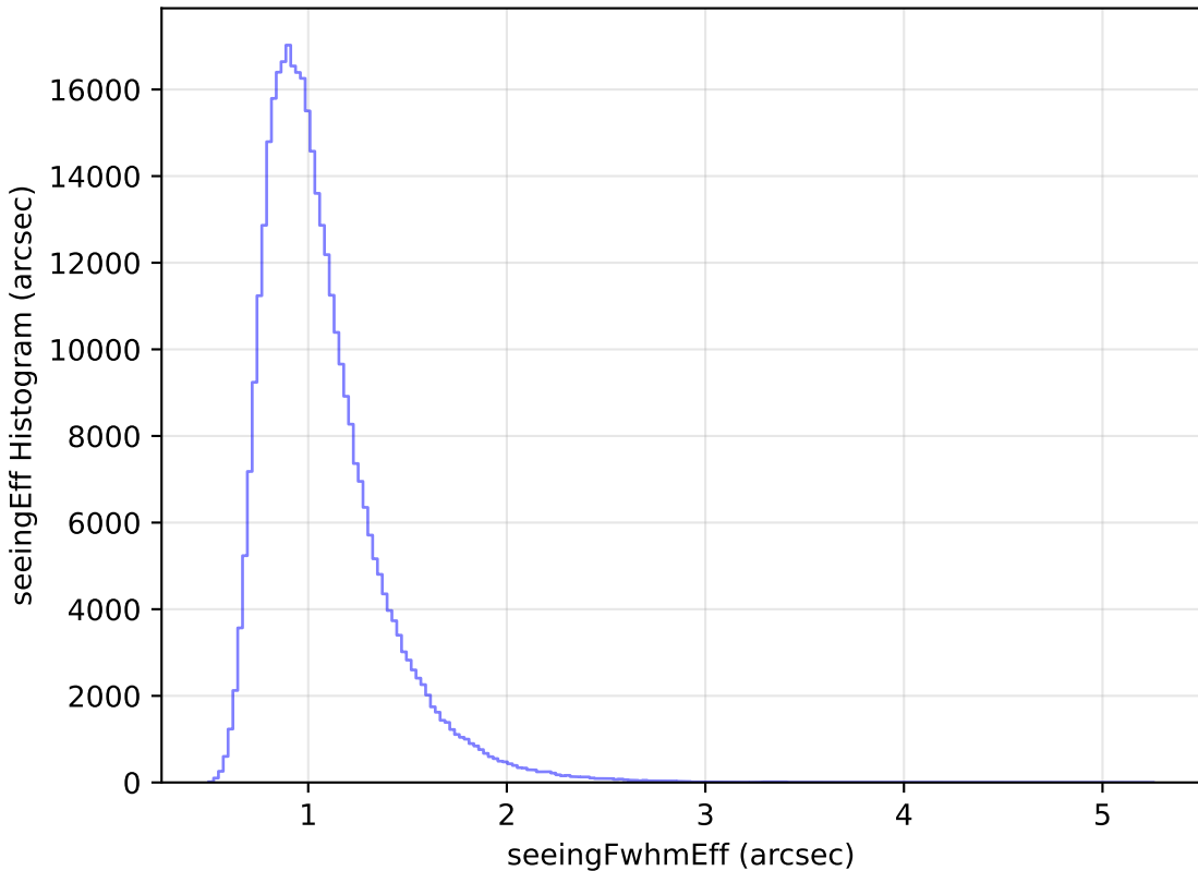
too_elab_r64_d3_ugrizy_v3.4_10yrs All sky y band: seeingEff Histogram
