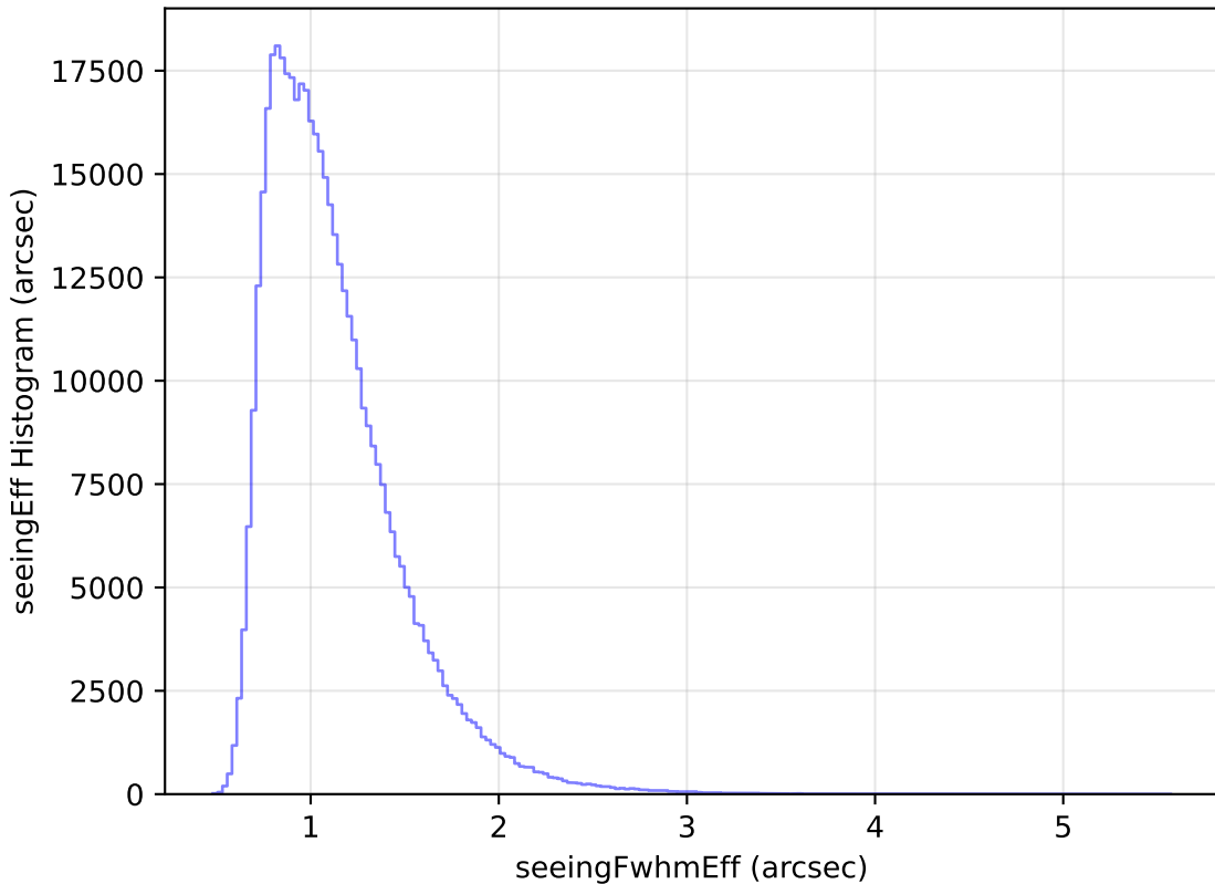
too_elab_r64_d3_ugrizy_v3.4_10yrs All sky r band: seeingEff Histogram
