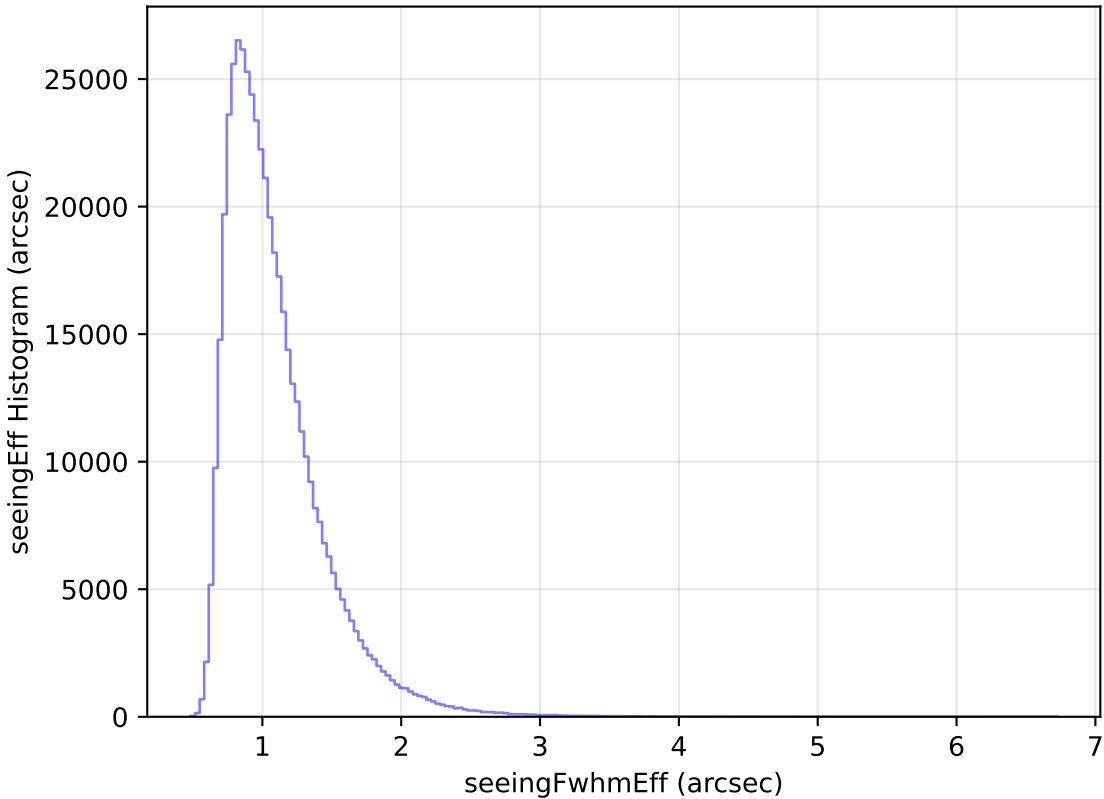
too_elab_r64_d3_ugrizy_v3.4_10yrs All sky i band: seeingEff Histogram
