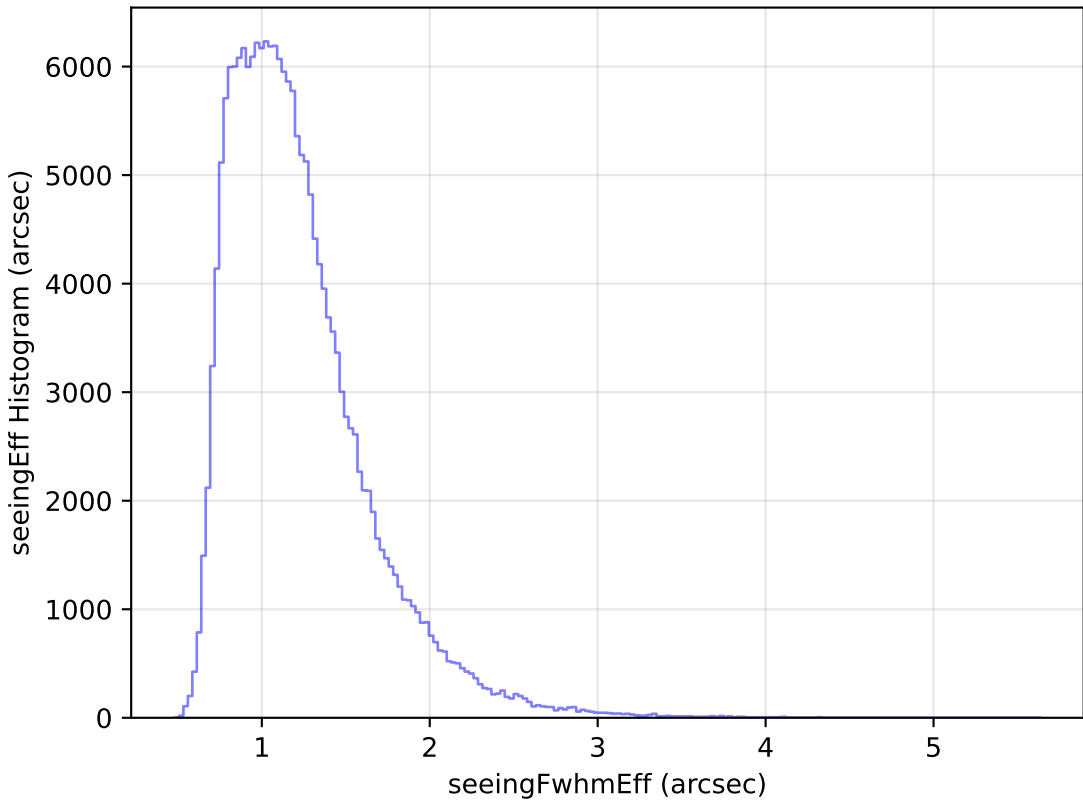
too_elab_r64_d3_ugrizy_v3.4_10yrs All sky g band: seeingEff Histogram
