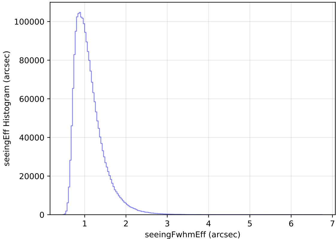
too_elab_r64_d3_ugrizy_v3.4_10yrs All sky all bands: seeingEff Histogram
