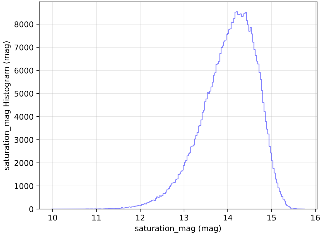
too_elab_r64_d3_ugrizy_v3.4_10yrs WFD z band: saturation_mag Histogram
