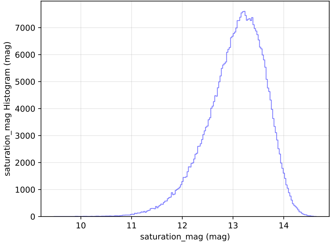
too_elab_r64_d3_ugrizy_v3.4_10yrs WFD y band: saturation_mag Histogram
