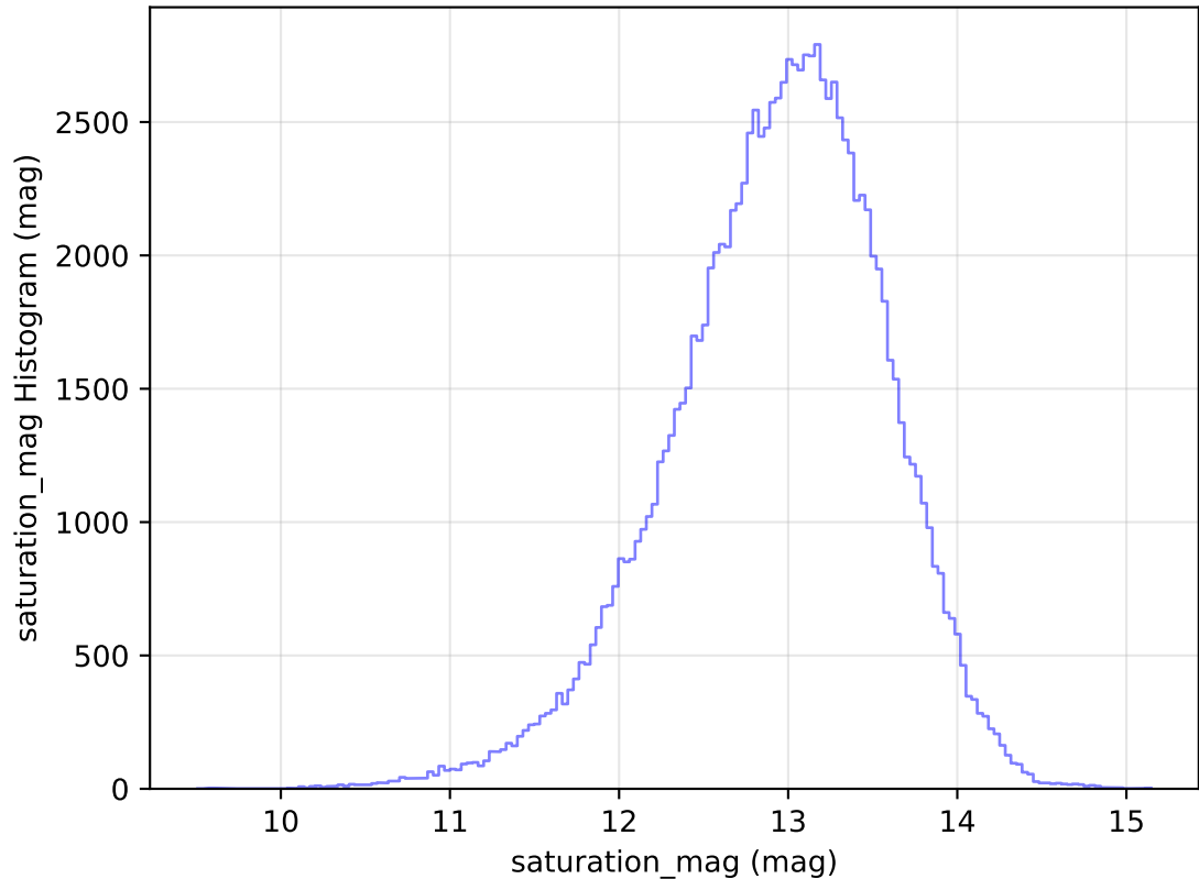
too_elab_r64_d3_ugrizy_v3.4_10yrs WFD u band: saturation_mag Histogram
