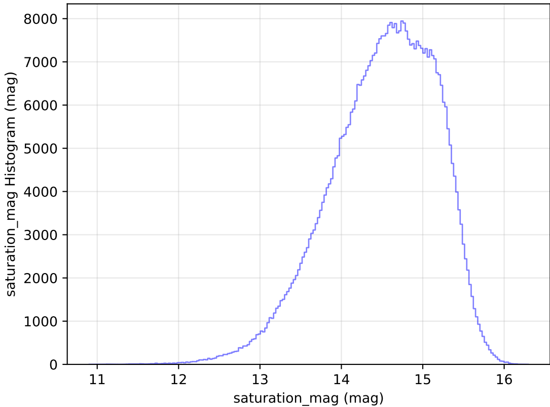
too_elab_r64_d3_ugrizy_v3.4_10yrs WFD r band: saturation_mag Histogram
