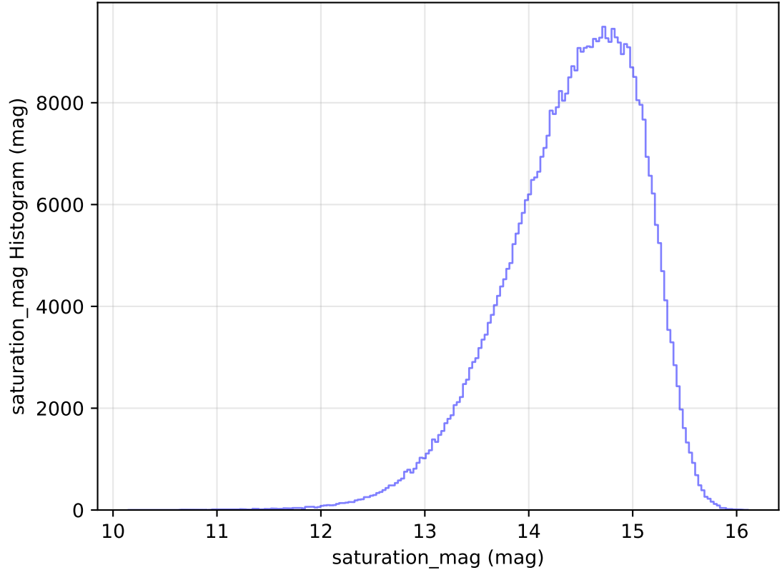
too_elab_r64_d3_ugrizy_v3.4_10yrs WFD i band: saturation_mag Histogram
