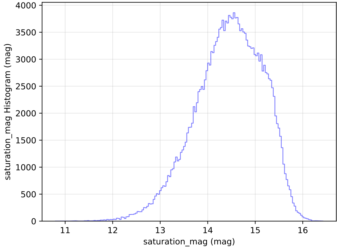
too_elab_r64_d3_ugrizy_v3.4_10yrs WFD g band: saturation_mag Histogram
