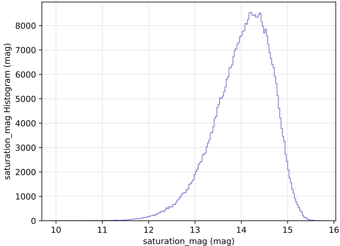
too_elab_r64_d3_ugrizy_v3.4_10yrs All sky z band: saturation_mag Histogram
