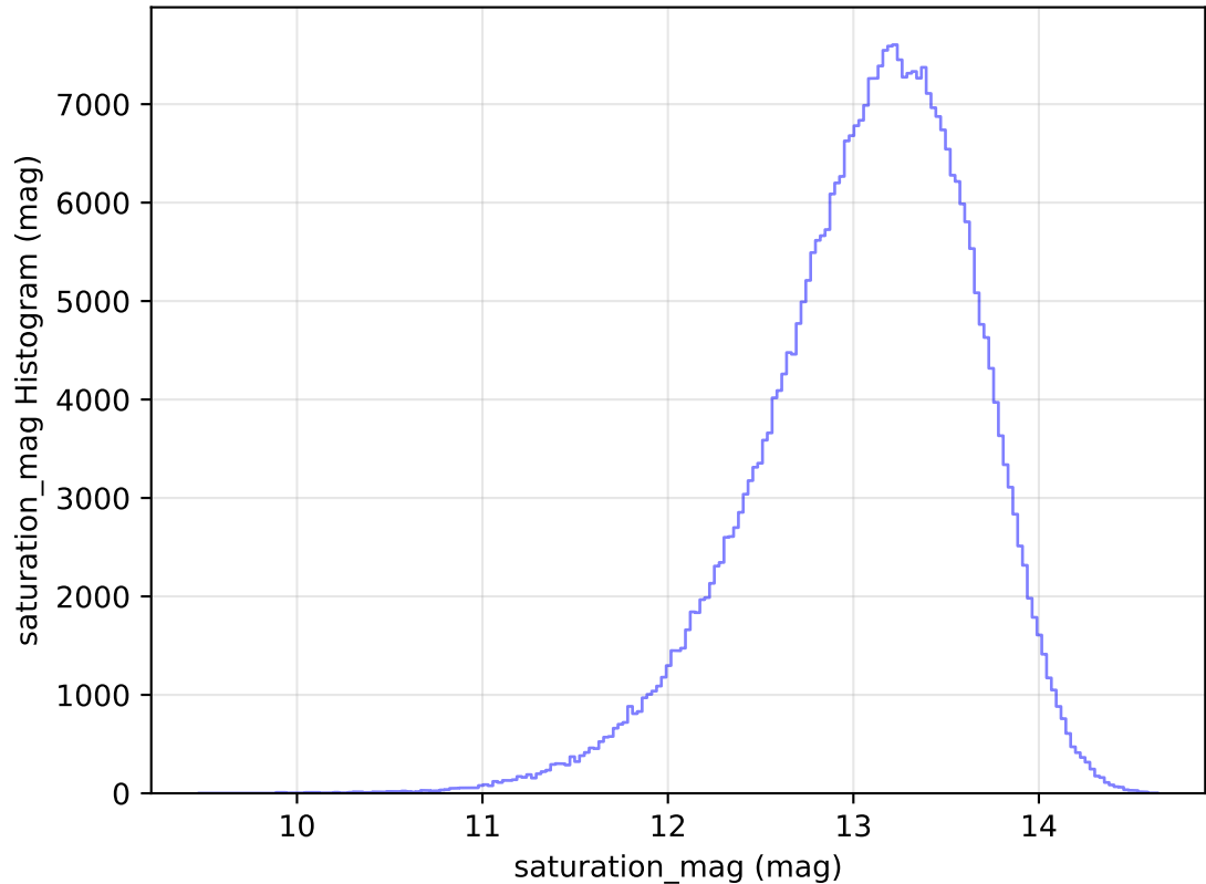
too_elab_r64_d3_ugrizy_v3.4_10yrs All sky y band: saturation_mag Histogram
