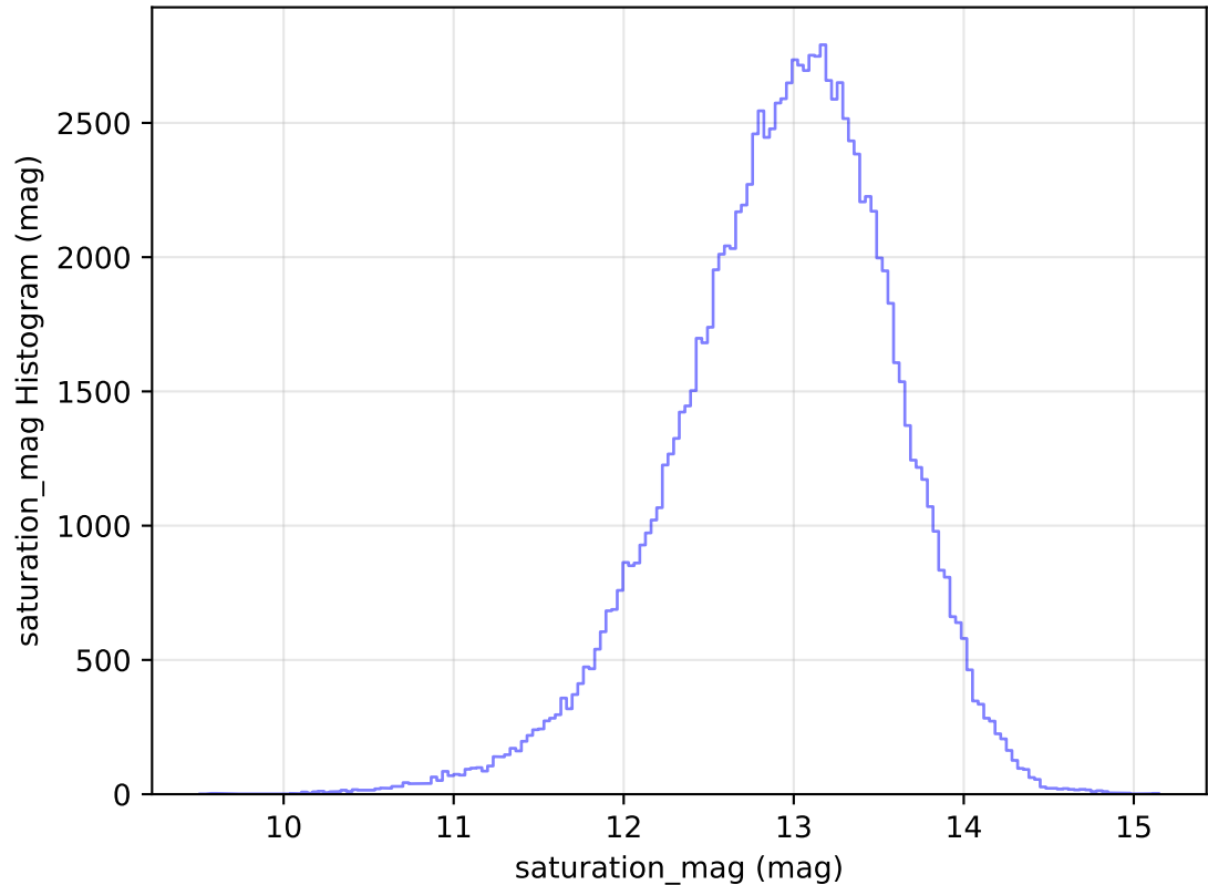
too_elab_r64_d3_ugrizy_v3.4_10yrs All sky u band: saturation_mag Histogram
