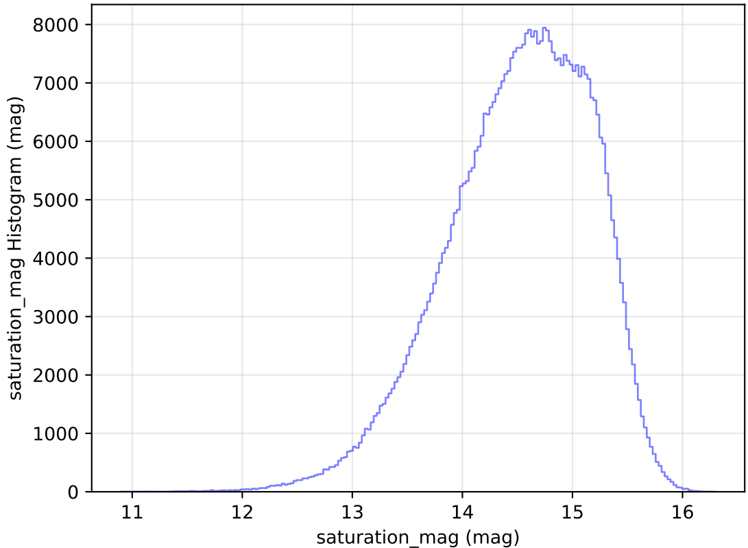
too_elab_r64_d3_ugrizy_v3.4_10yrs All sky r band: saturation_mag Histogram
