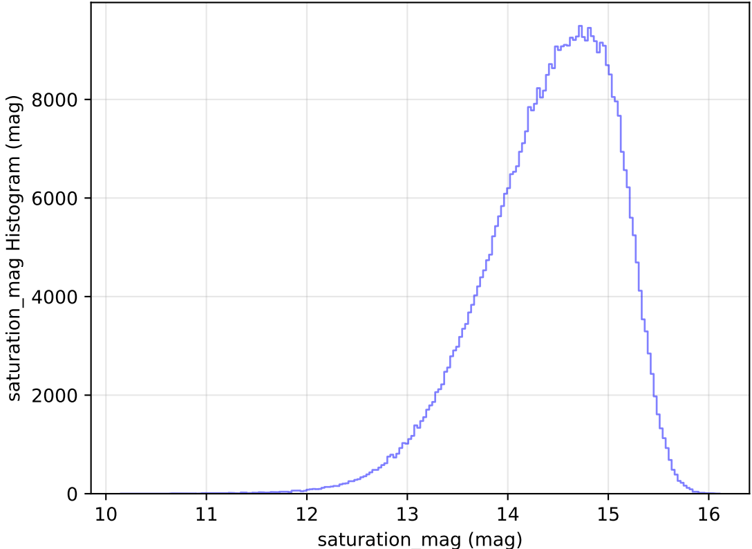
too_elab_r64_d3_ugrizy_v3.4_10yrs All sky i band: saturation_mag Histogram
