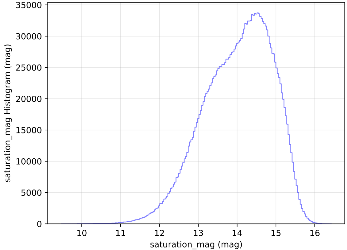
too_elab_r64_d3_ugrizy_v3.4_10yrs All sky all bands: saturation_mag Histogram
