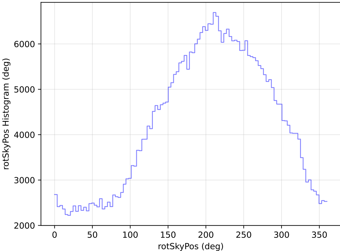
too_elab_r64_d3_ugrizy_v3.4_10yrs WFD z band: rotSkyPos Histogram
