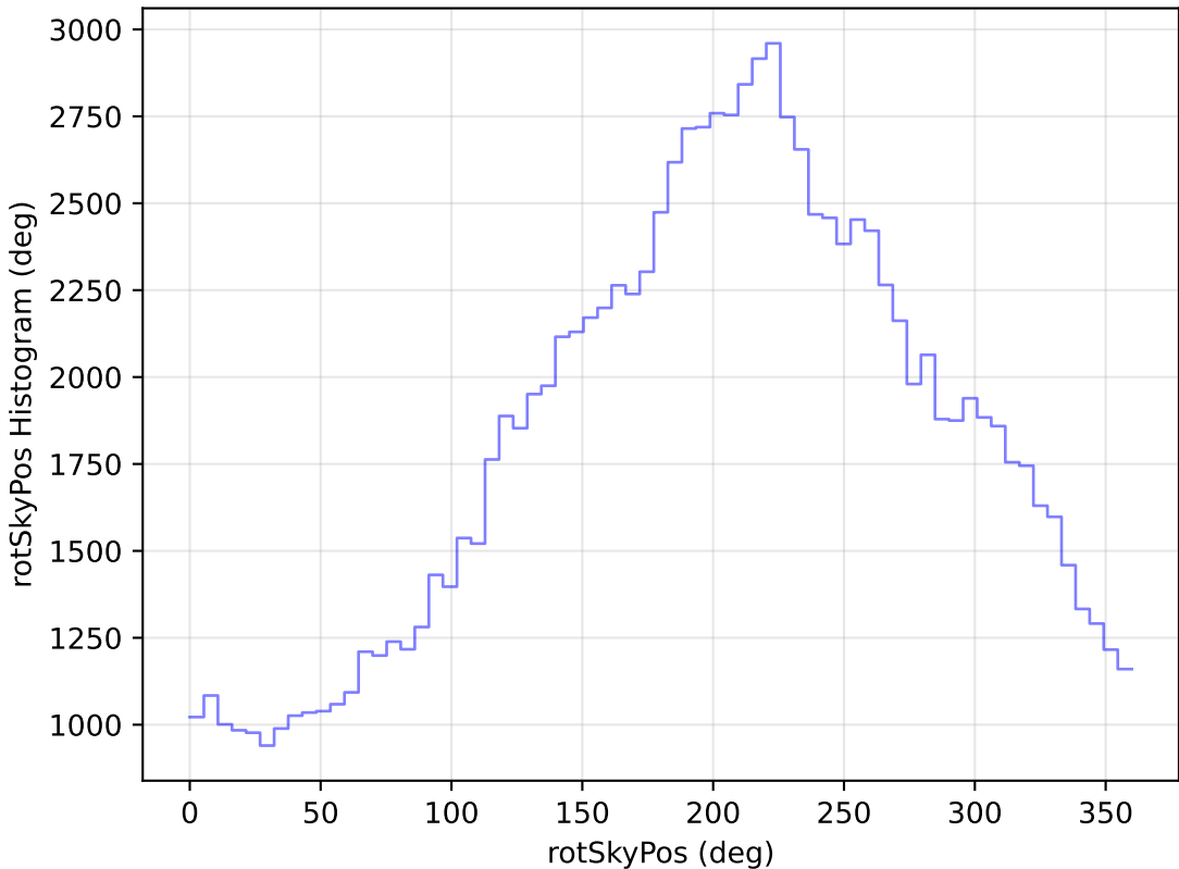
too_elab_r64_d3_ugrizy_v3.4_10yrs WFD u band: rotSkyPos Histogram
