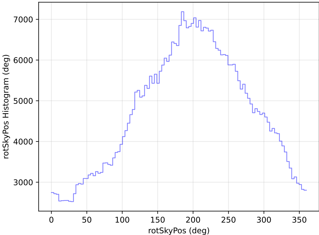
too_elab_r64_d3_ugrizy_v3.4_10yrs WFD r band: rotSkyPos Histogram
