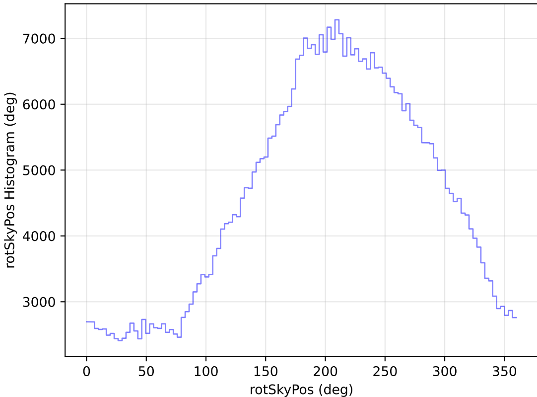
too_elab_r64_d3_ugrizy_v3.4_10yrs WFD i band: rotSkyPos Histogram
