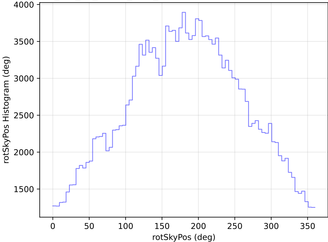
too_elab_r64_d3_ugrizy_v3.4_10yrs WFD g band: rotSkyPos Histogram
