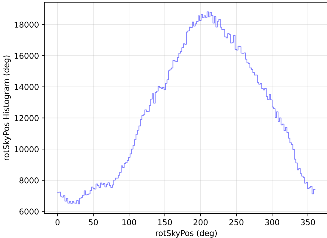
too_elab_r64_d3_ugrizy_v3.4_10yrs WFD all bands: rotSkyPos Histogram
