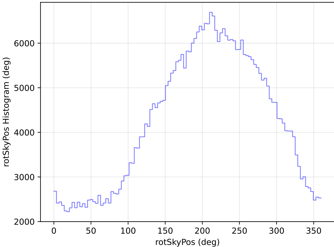
too_elab_r64_d3_ugrizy_v3.4_10yrs All sky z band: rotSkyPos Histogram
