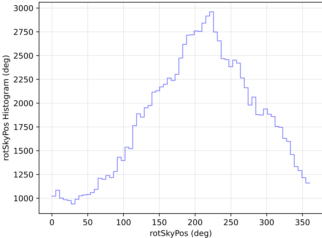
too_elab_r64_d3_ugrizy_v3.4_10yrs All sky u band: rotSkyPos Histogram
