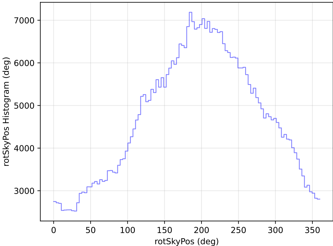
too_elab_r64_d3_ugrizy_v3.4_10yrs All sky r band: rotSkyPos Histogram
