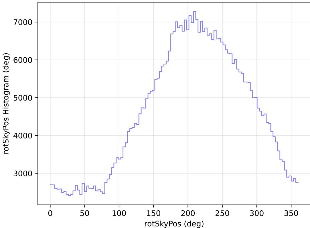
too_elab_r64_d3_ugrizy_v3.4_10yrs All sky i band: rotSkyPos Histogram
