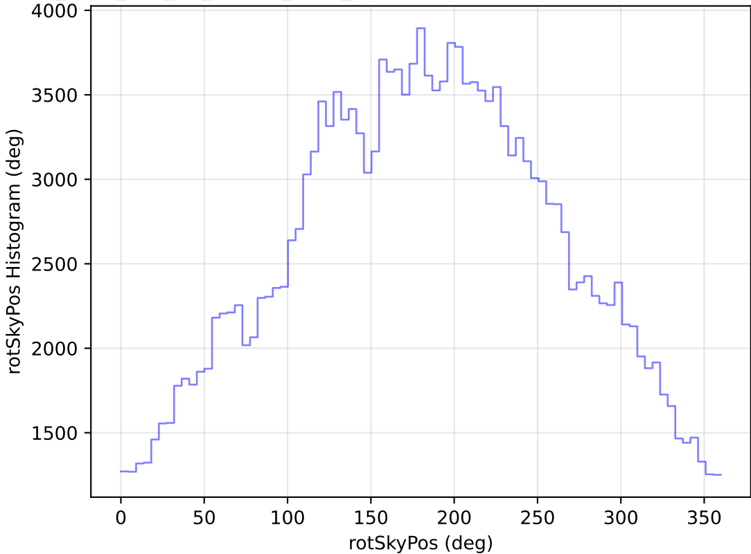
too_elab_r64_d3_ugrizy_v3.4_10yrs All sky g band: rotSkyPos Histogram
