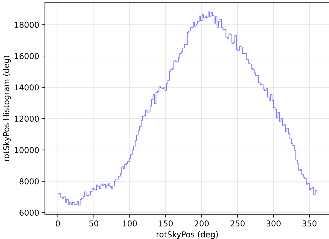
too_elab_r64_d3_ugrizy_v3.4_10yrs All sky all bands: rotSkyPos Histogram
