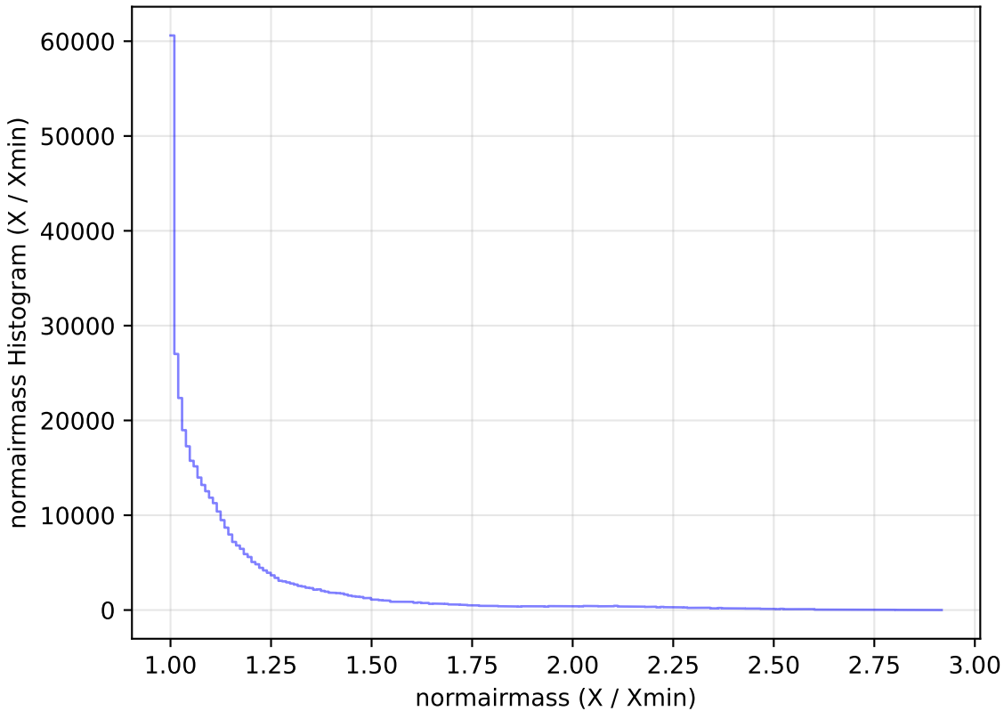
too_elab_r64_d3_ugrizy_v3.4_10yrs WFD z band: normairmass Histogram
