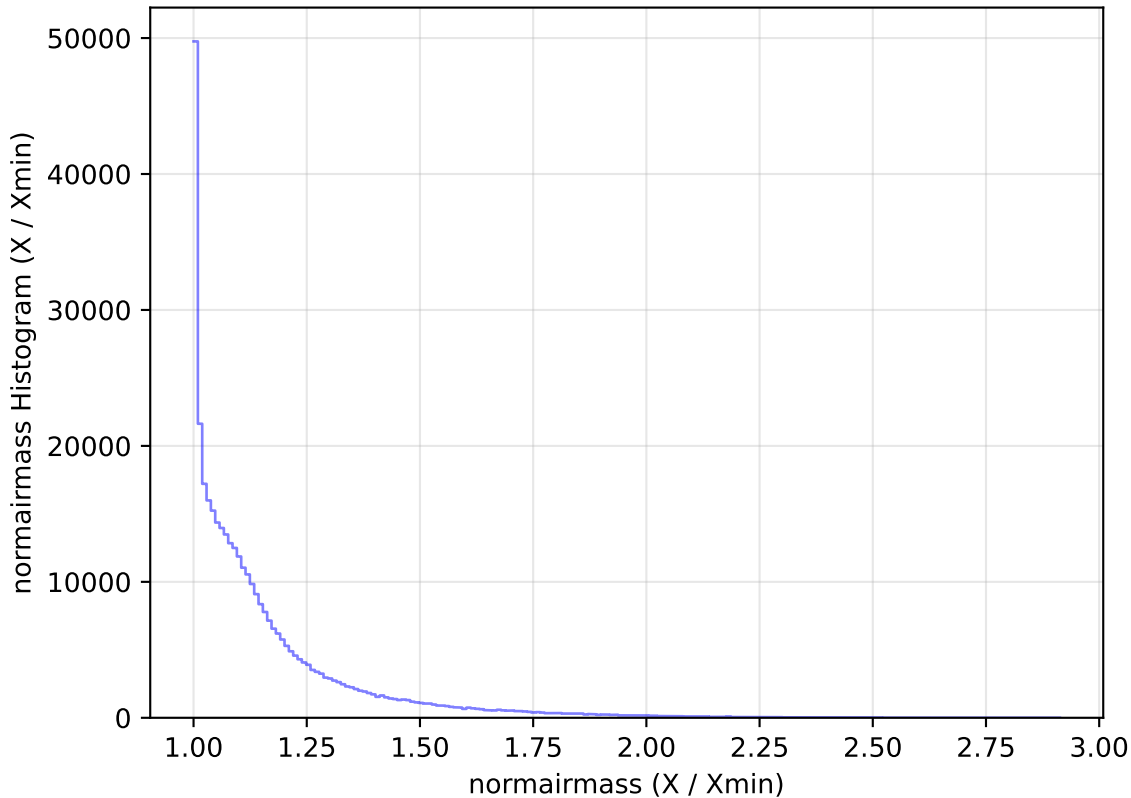
too_elab_r64_d3_ugrizy_v3.4_10yrs WFD y band: normairmass Histogram
