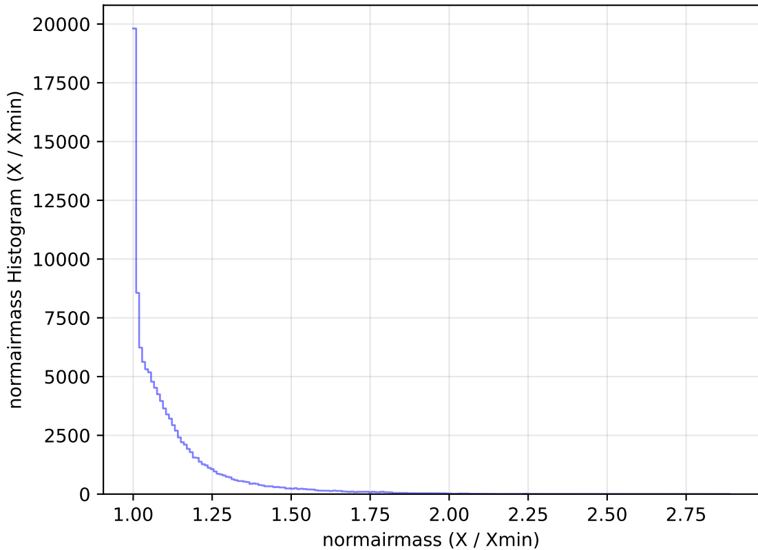
too_elab_r64_d3_ugrizy_v3.4_10yrs WFD u band: normairmass Histogram
