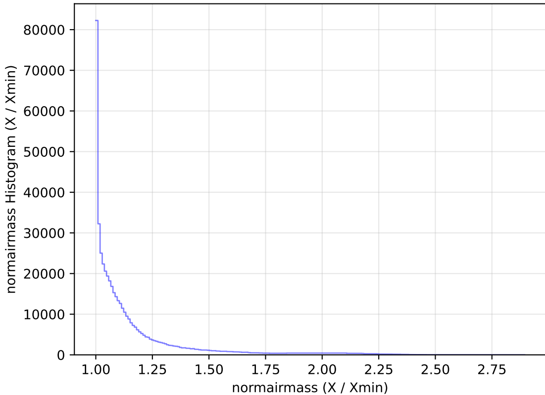
too_elab_r64_d3_ugrizy_v3.4_10yrs WFD r band: normairmass Histogram
