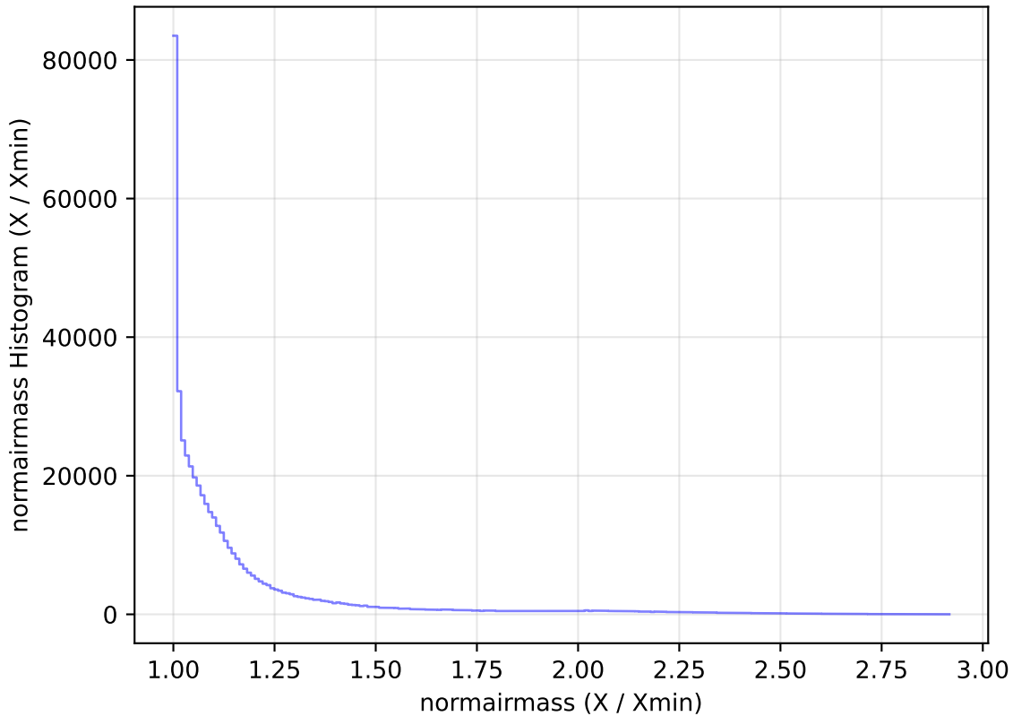
too_elab_r64_d3_ugrizy_v3.4_10yrs WFD i band: normairmass Histogram
