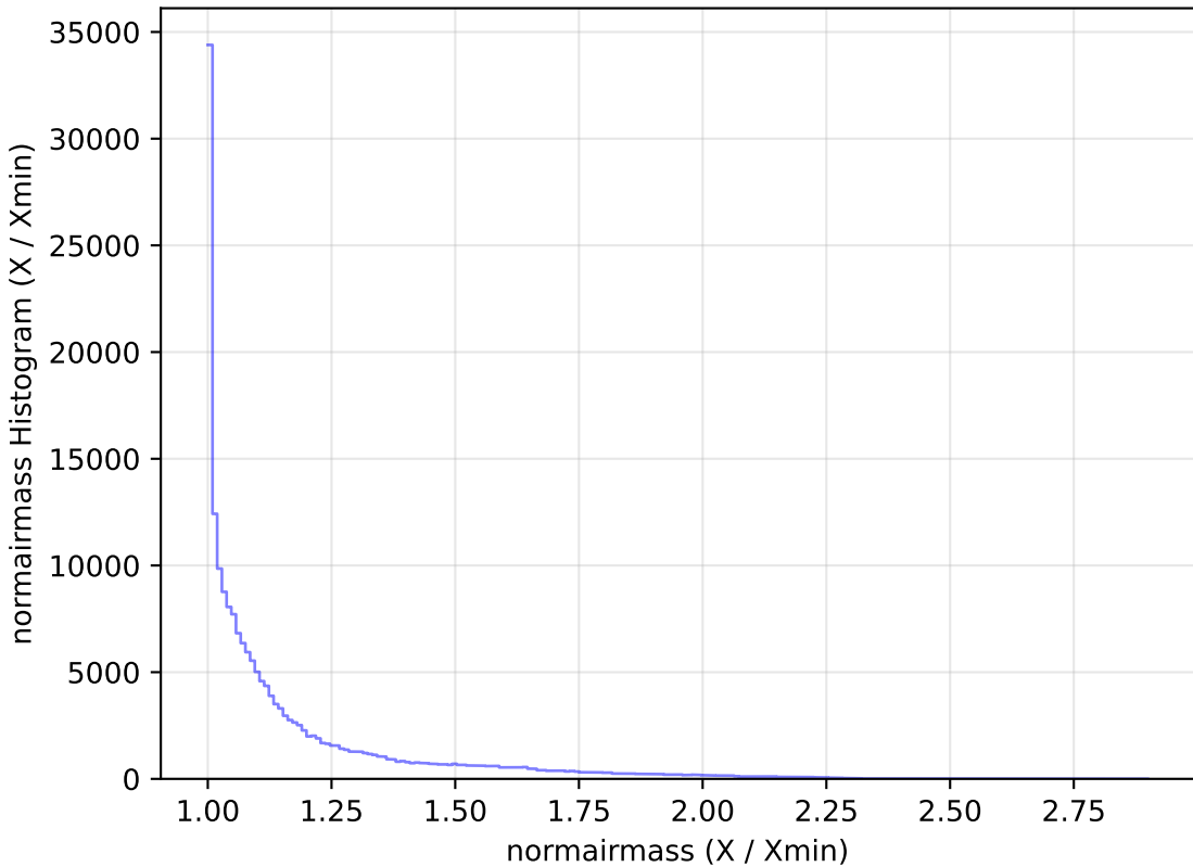
too_elab_r64_d3_ugrizy_v3.4_10yrs WFD g band: normairmass Histogram
