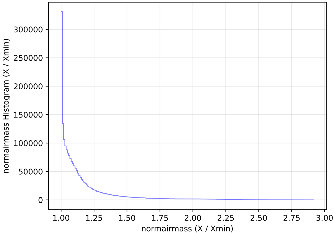
too_elab_r64_d3_ugrizy_v3.4_10yrs WFD all bands: normairmass Histogram
