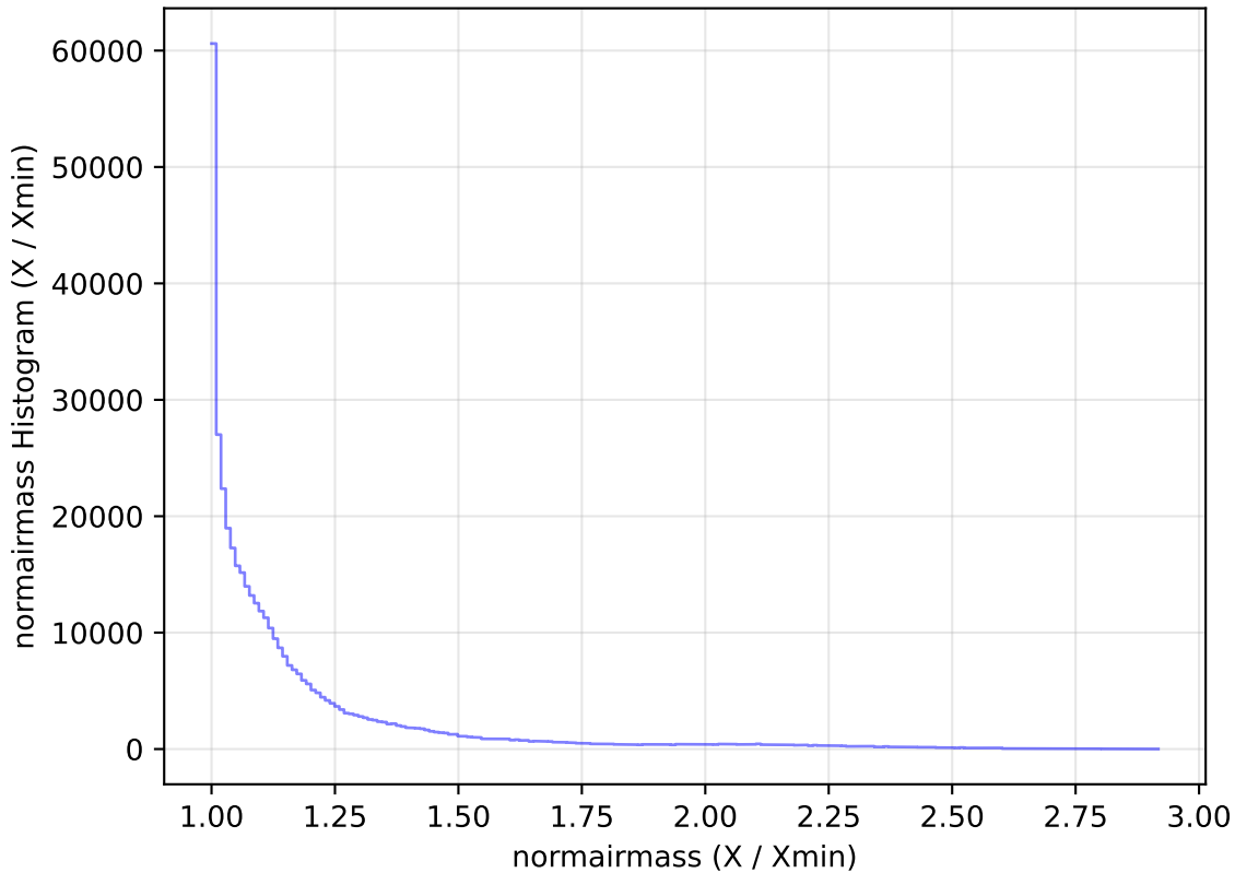
too_elab_r64_d3_ugrizy_v3.4_10yrs All sky z band: normairmass Histogram
